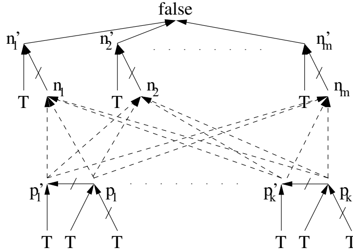
Figure 2: A translation from satisfiability to prioritized default logic
