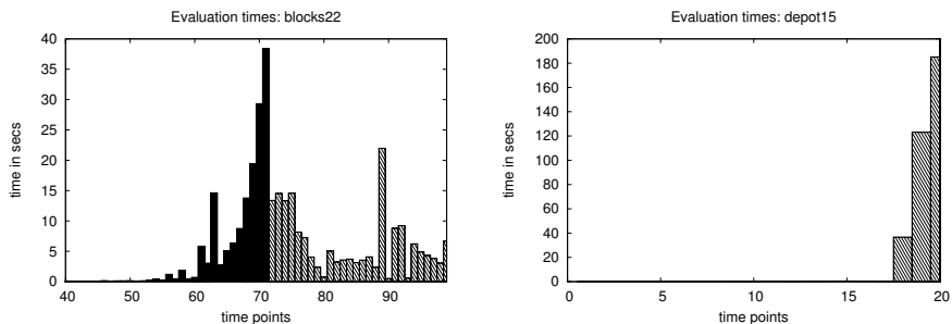
Figure 19.2. SAT solver runtimes for two problem instances and different plan lengths
