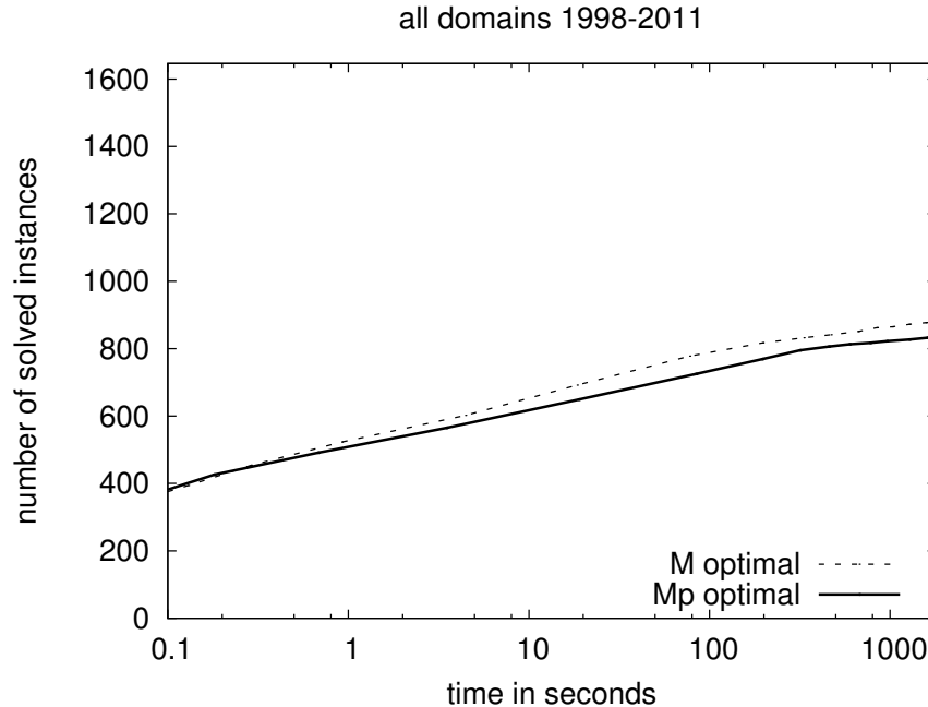
Figure 10: Number of instances solved in a given time with the sequential strategy
